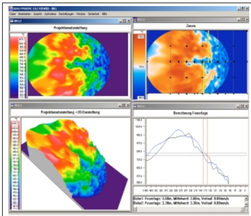
Pictures above: Thermal images of the whole surface of the great (fuel bed). Location of the area with the maximum heat release (main combustion zone). Image with the border line of the burning area and the burned mass with final cooling zone
